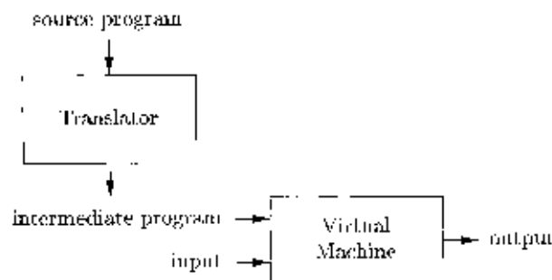
Figure 1.1: A hybrid compiler
