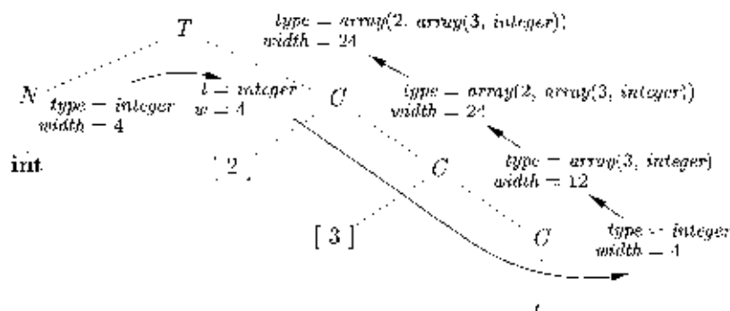
Figure 6.16: Syntax-directed translation of array types
