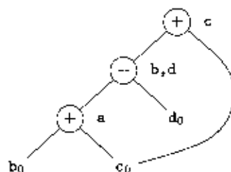
Figure 8.12: DAG for basic block in Example 8.10
