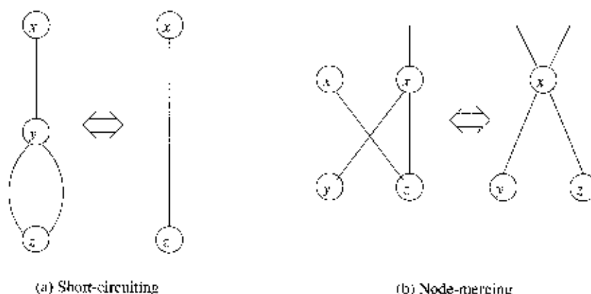
Figure 12.32: Transformations on BDD's
