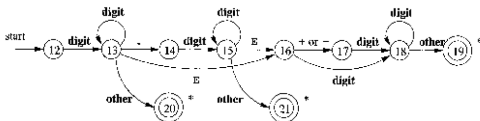
Figure 3.16: A transition diagram for unsigned numbers
