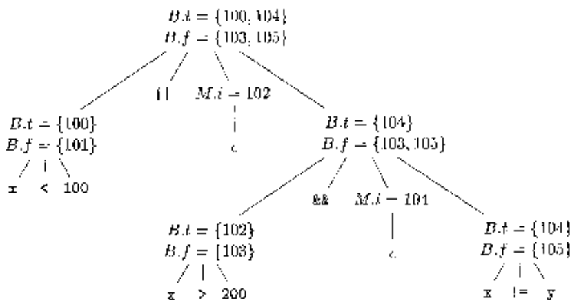
Figure 6.14: Annotated parse tree for x < 100 \mid \mid x > 200 \&\& x \neq y
