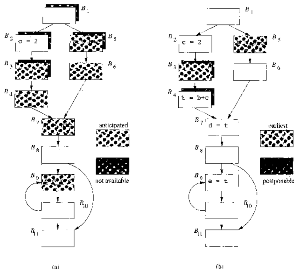
Figure 9.33: Flow graph of Example 9.30
