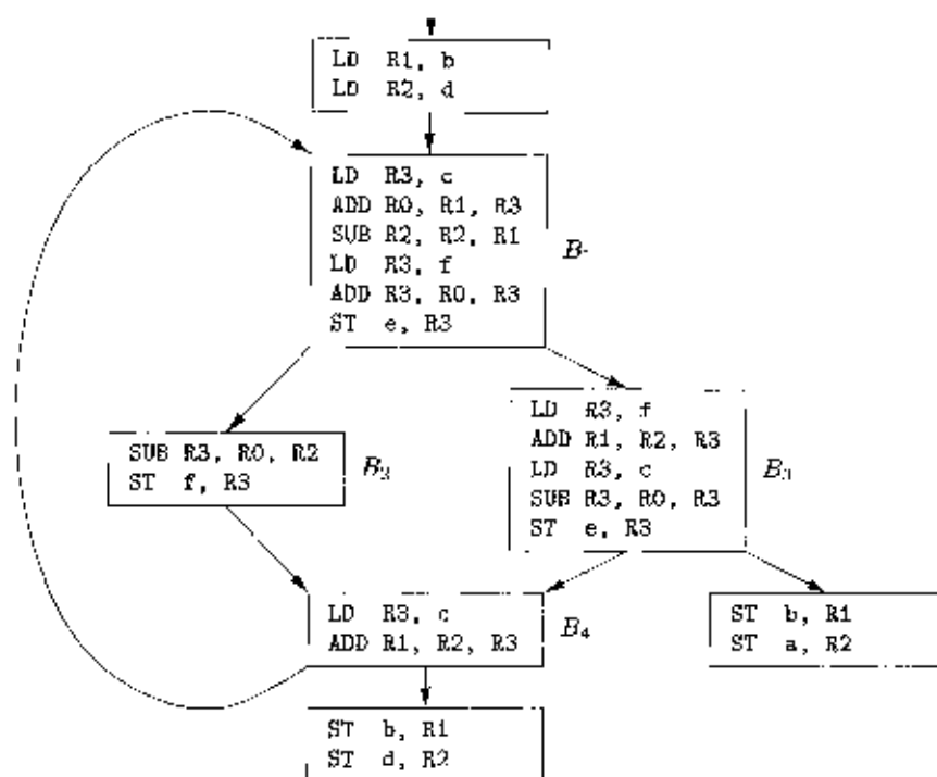
Figure 8.18: Code sequence using global register assignment
