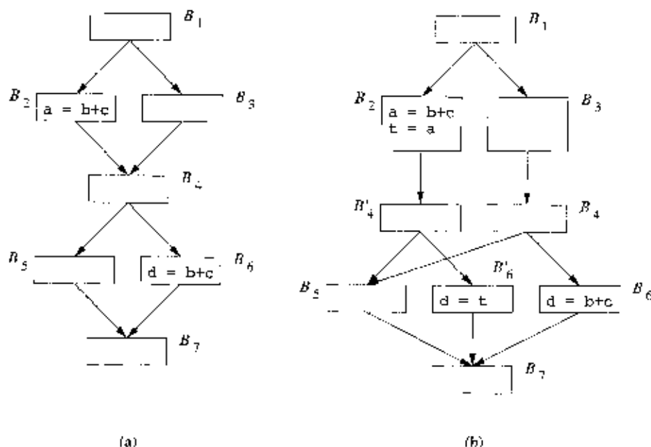
Figure 9.32: Code duplication to eliminate redundancies
