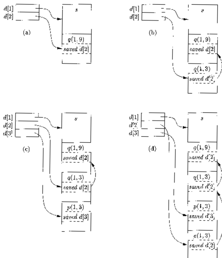
Figure 7.14: Maintaining the display
