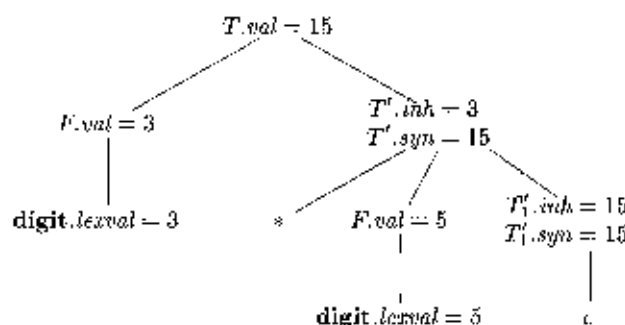
Figure 5.5: Annotated parse tree for 3 * 5
