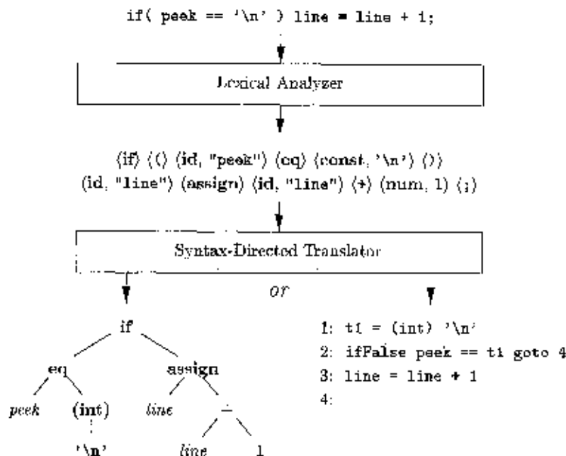
Figure 2.46: Two possible translations of a statement.
