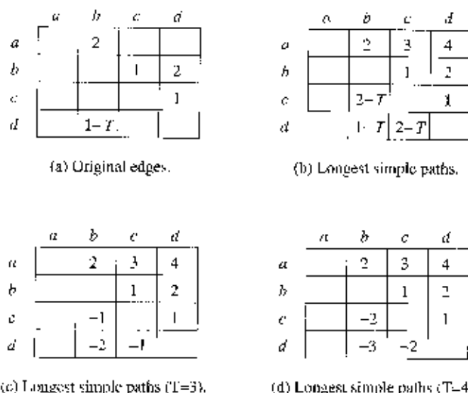
Figure 10.28: Transitive dependences in Example 10.20
