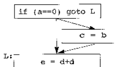
(a) Source program
