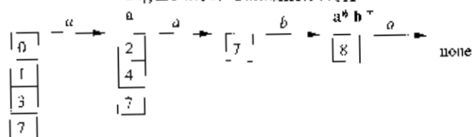
Figure 3.52: Combined NFA
