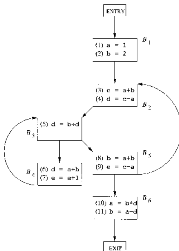
Figure 9.10: Flow graph for Exercise 9.1.1
