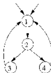
Figure 9.16: Two loops with the same header
