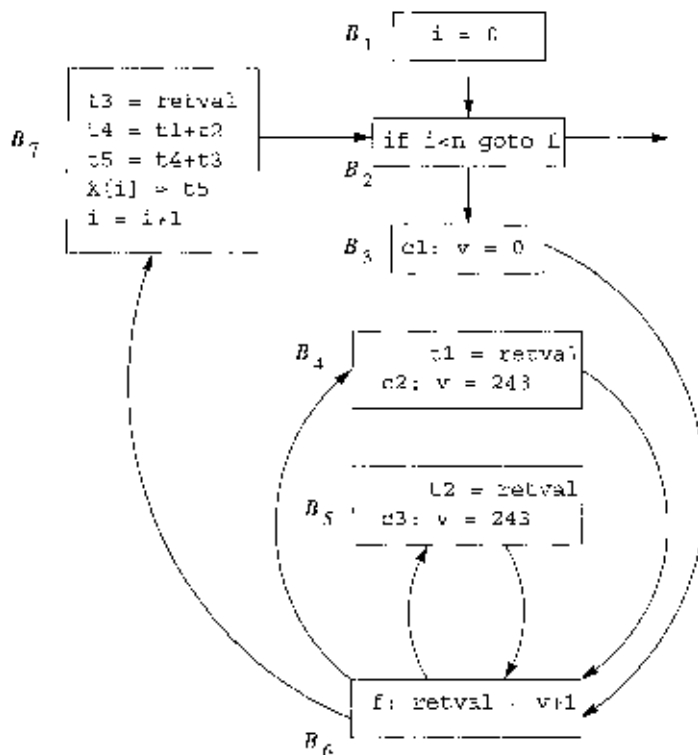
Figure 12.4: The control-flow graph for Fig. 12.3, treating function calls as control flow
