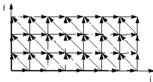
(b) Data dependencies in the code.
