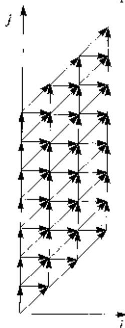
Figure 11.51: Fully permutable version of the code Fig. 11.50
