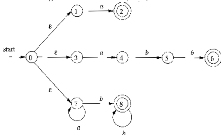
Figure 3.51: NFA's for a , abb , and a^*b^+
