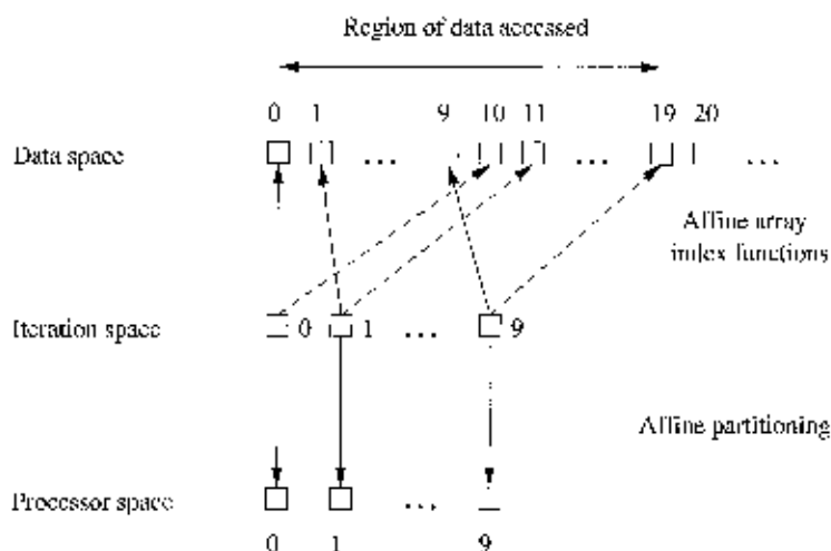
Figure 11.4: Iteration, data, and processor space for Example 11.4
