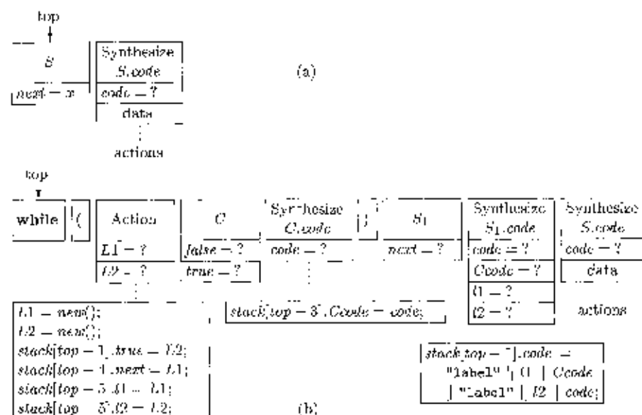
Figure 5.35: Expansion of S with synthesized attributes constructed on the stack
