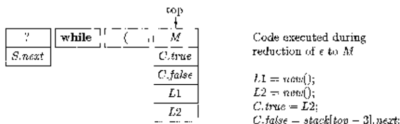
Figure 5.36: LR parsing stack after reduction of c to M
