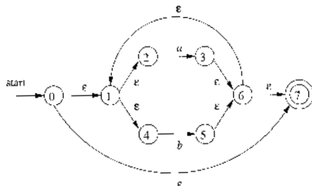
Figure 3.45: NFA for r_5
