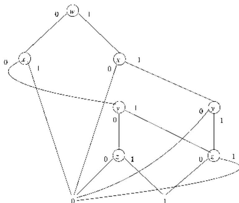
Figure 12.31: A binary decision diagram
