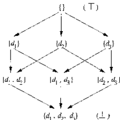
Figure 9.22: Lattice of subsets of definitions
