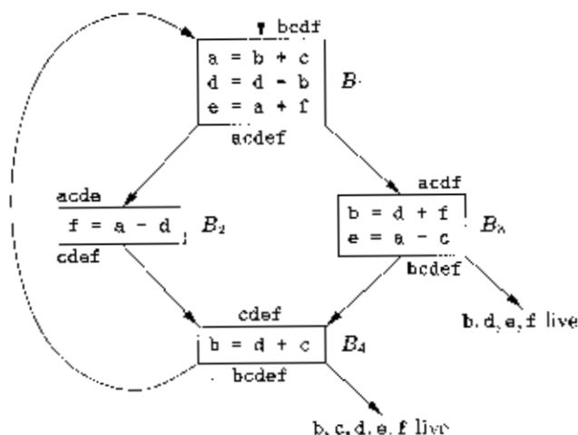
Figure 8.17: Flow graph of an inner loop
