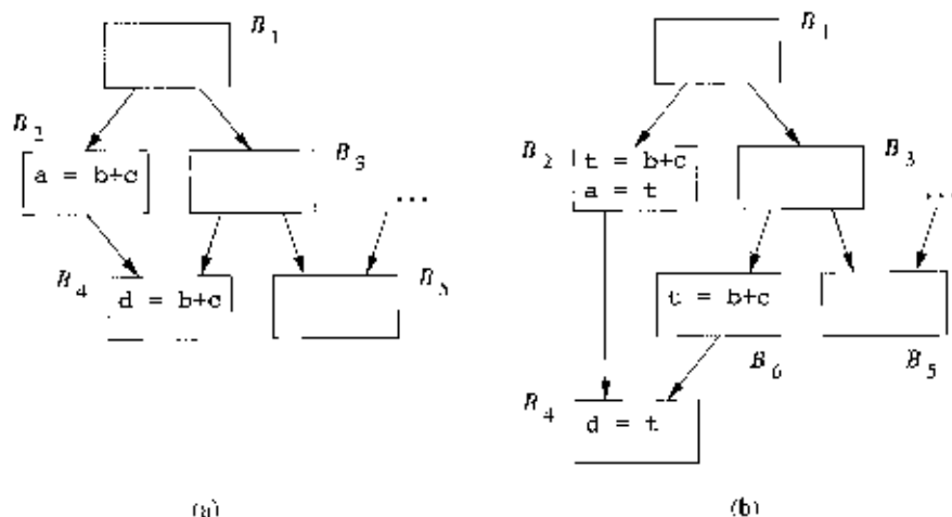
Figure 9.31: B_2 \rightarrow B_4 is a critical edge
