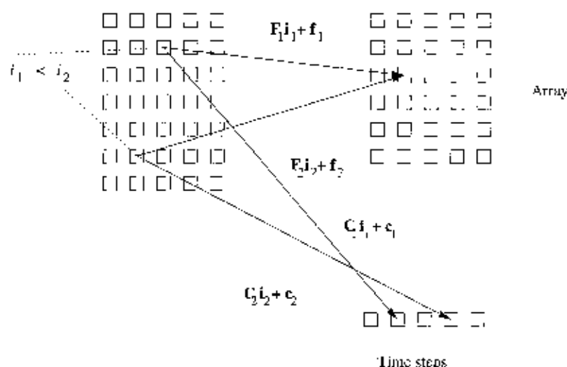
Figure 11.54: Time-Partition Constraints
